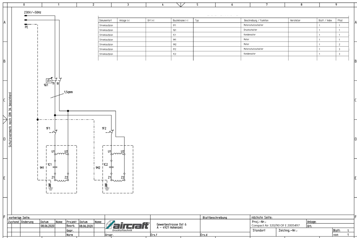
Abb. 20: Elektro-Schaltplan COMPACT AIR 320/90 V OF E
