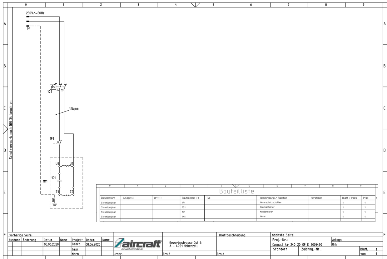
Abb. 19: Elektro-Schaltplan COMPACT-AIR 240/20 OF E, 240/40 V OF E, 320/24 OF E und Silence 231/20 OF E
