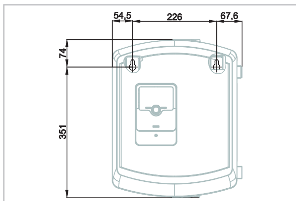
Abb. 5: Wandmontage
